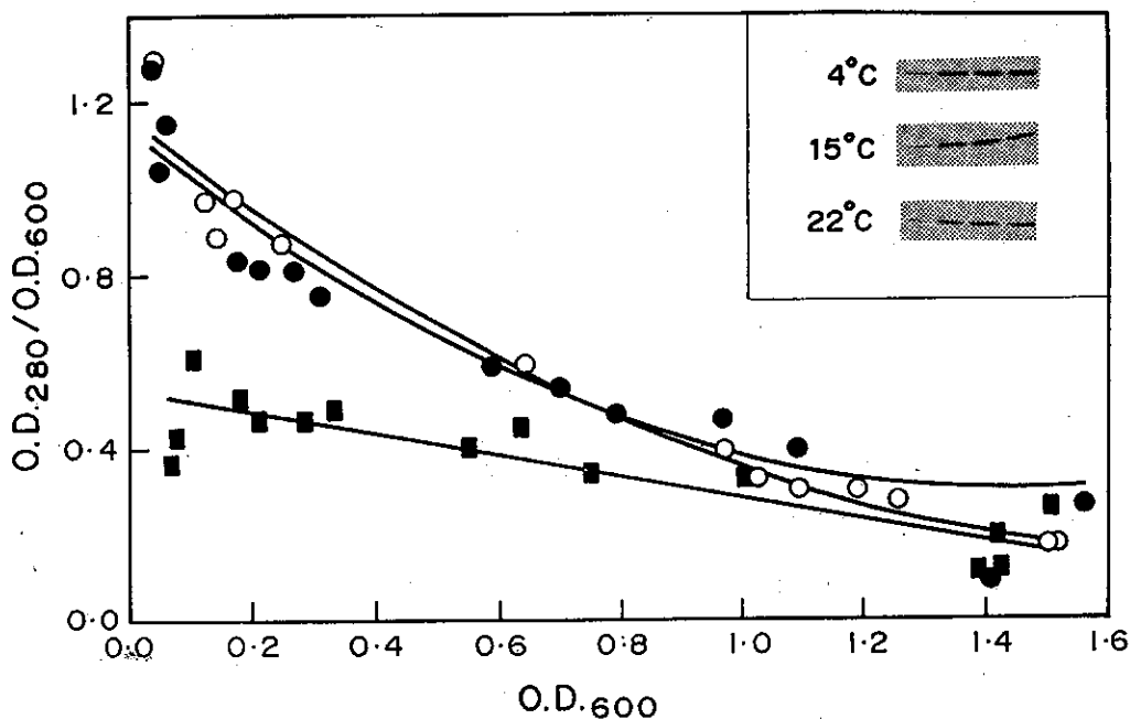
Figure 5. Production of extracellular protease by the antarctic psychrotrophic yeast C. humicola at various temperatures (4°C, ○; 15°C, ●; and 22°C, ■). The ratio, \text{OD}_{280}/\text{OD}_{600} is a measure of protease activity per a constant number of cells which has been plotted against \text{OD}_{600} to indicate the stage of growth of cells. The inset shows silver nitrate stained protein bands corresponding to the protease which was secreted into the growth medium. For further details, see Ray et al (1992).
